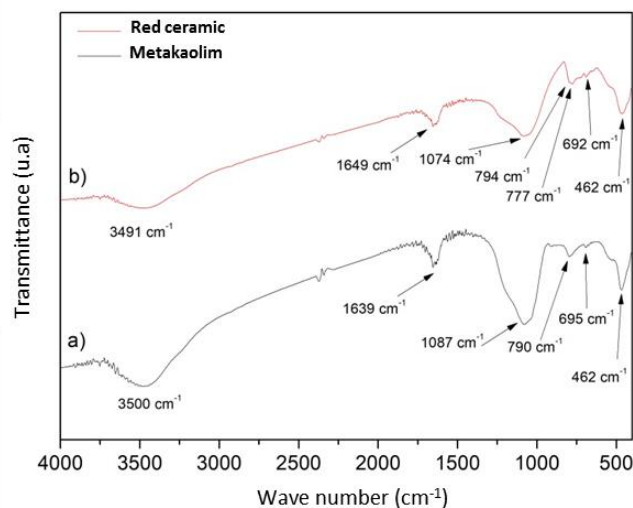
Figure 6. FTIR: a)metakaolim and b)red ceramic used in the manufacturing of polymers.
